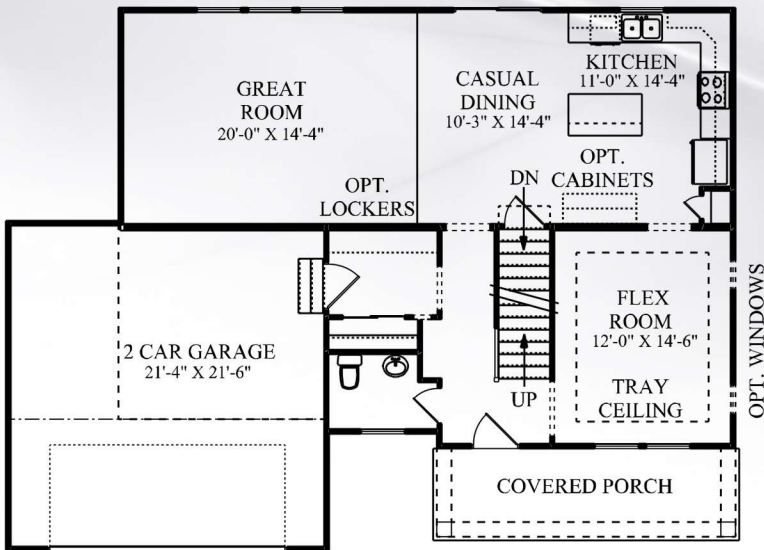
Main Floor - 1045 Square Feet
